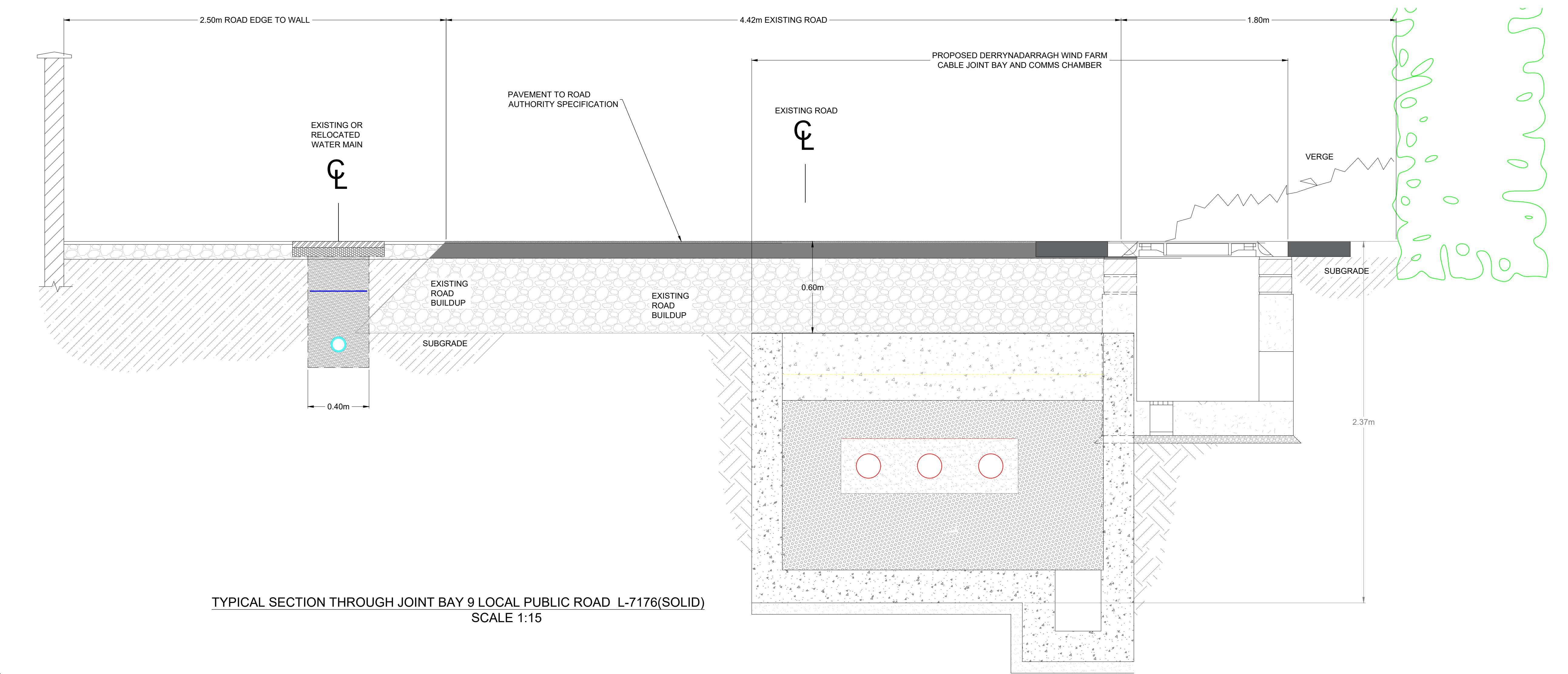
TYPICAL SECTION THROUGH LOCAL PUBLIC ROAD L-7176(SOLID) SCALE 1:15
